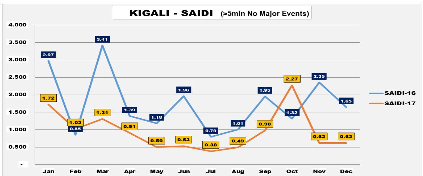
Fig – 1: Comparison of SAIDI (2016-2017) (No Major Events)
