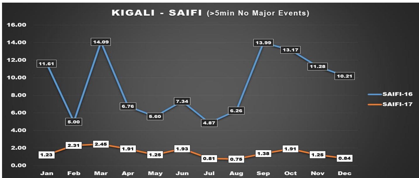
Fig – 2: Comparison of SAIFI (2016-2017) (No Major Events)
